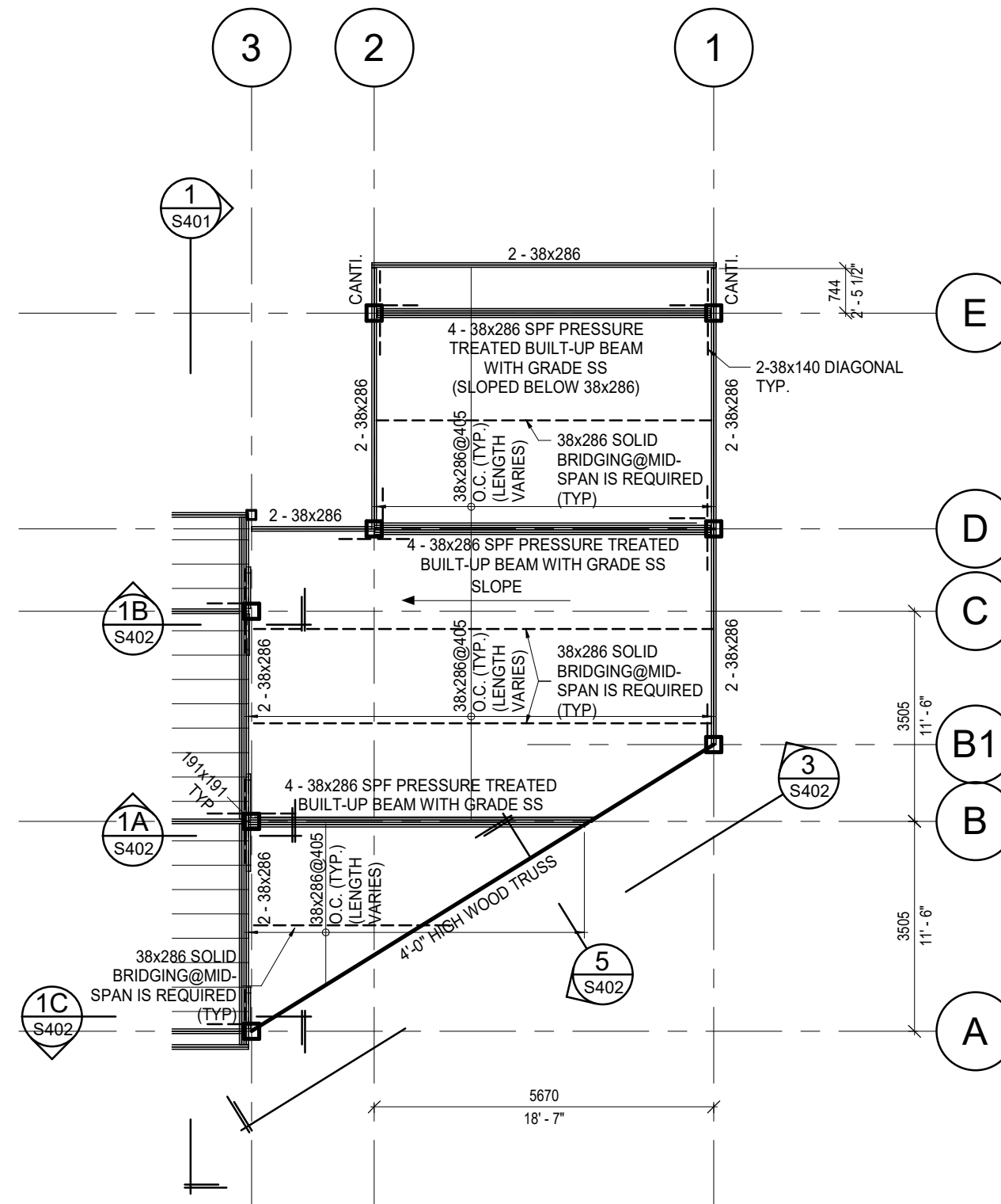
3 HIGH ROOF CANOPY 1 S201 1 : 100
